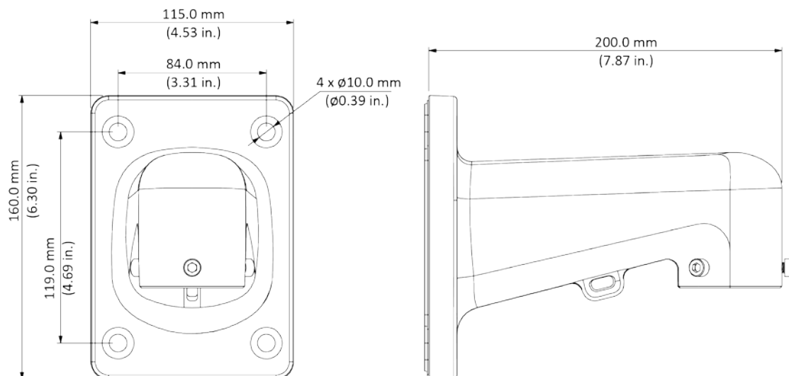
Figure 3-2: PFB30W Wall Mount Dimensions
