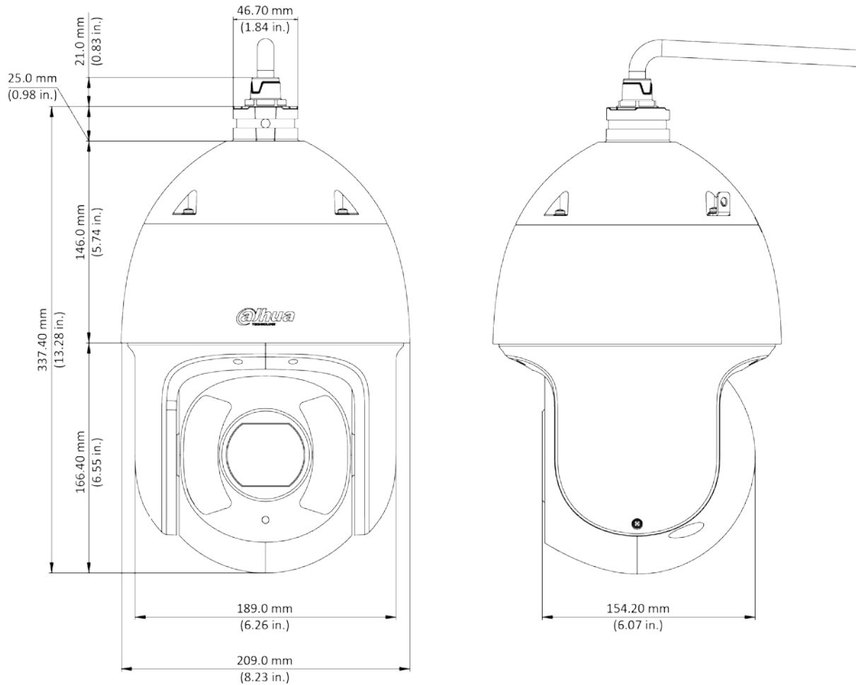
Figure 3-1: Dimensions for 6CE230UNI
