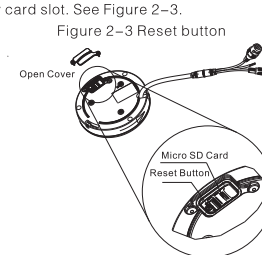
Figure 2-3 Reset button
