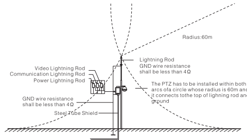
Appendix figure 1-1 Outdoor installation
