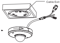
Figure 3-5 Rotating the speed dome pedestal
