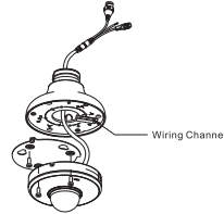
Figure 4-4 Installing the mounting plate
