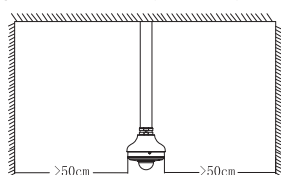
Figure 4-8 Installation position requirement
