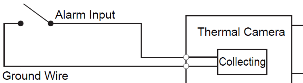
Figure 5-2 Alarm input
