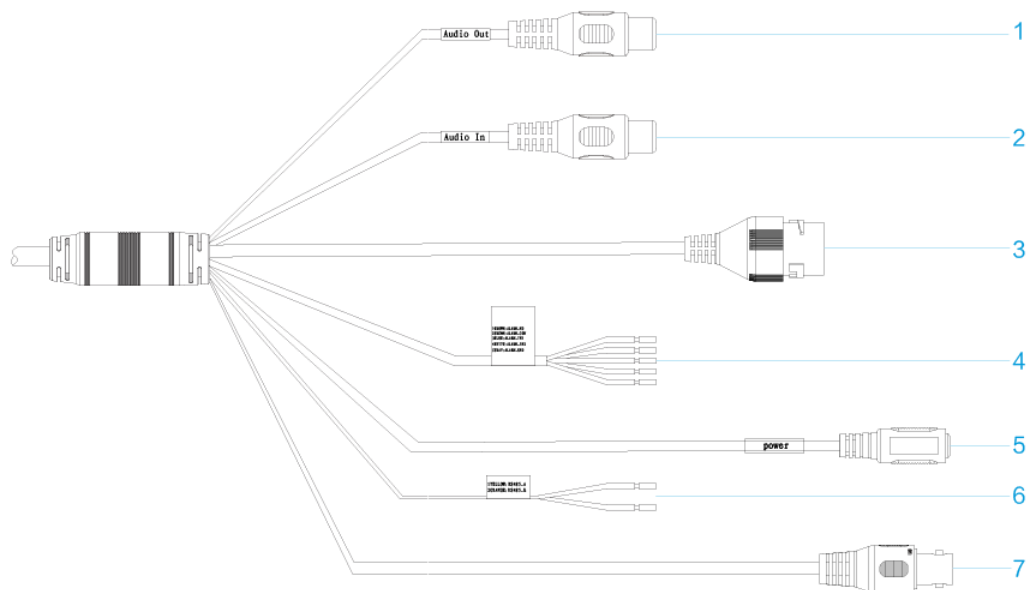
Figure 2-2 Cable ports
