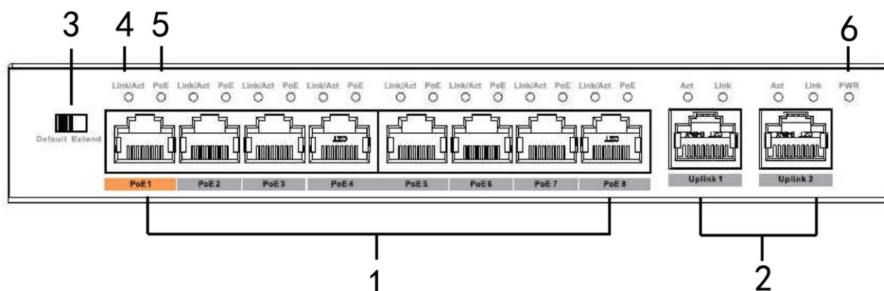
Figure 2-1 Front panel
