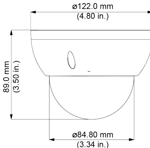
Figure 3-1: Dimensions
